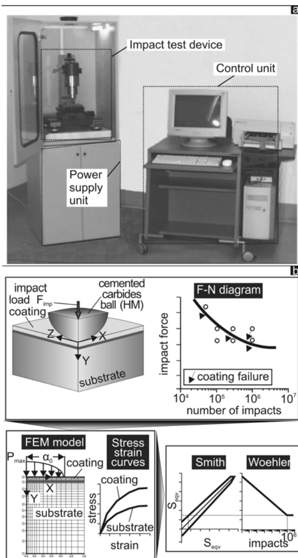
Figure 3: The impact tester working principle and its FEM simulation.
