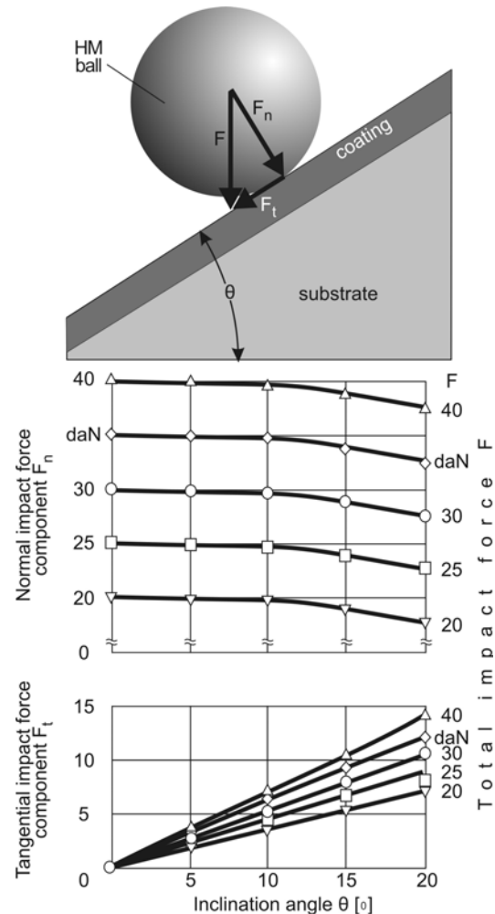
Figure 6: Normal and tangential force components over the applied impact load versus the inclination angle \theta .
