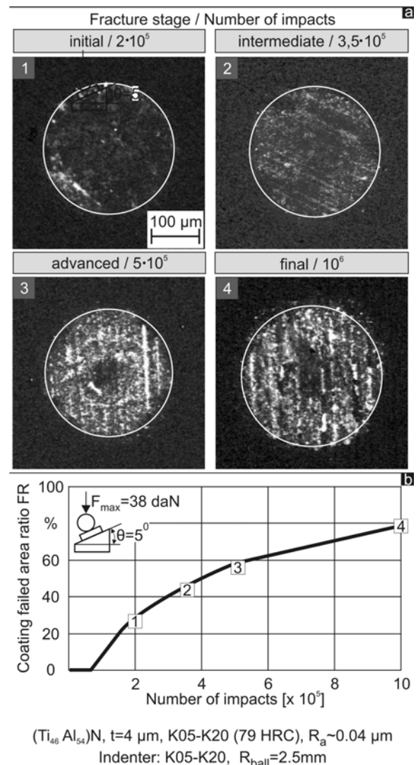
Figure 10: Elaboration of a coating removal propagation diagram.
